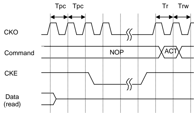
Figure 1-32 SDRAM Power-Down Mode Timing (CKO Stopped)
