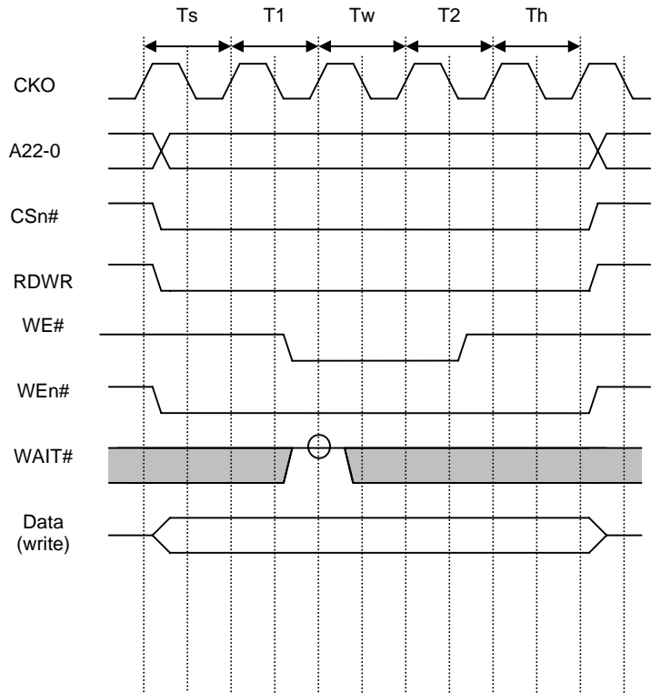
Figure 1-12 Byte Control SRAM Write Timing
