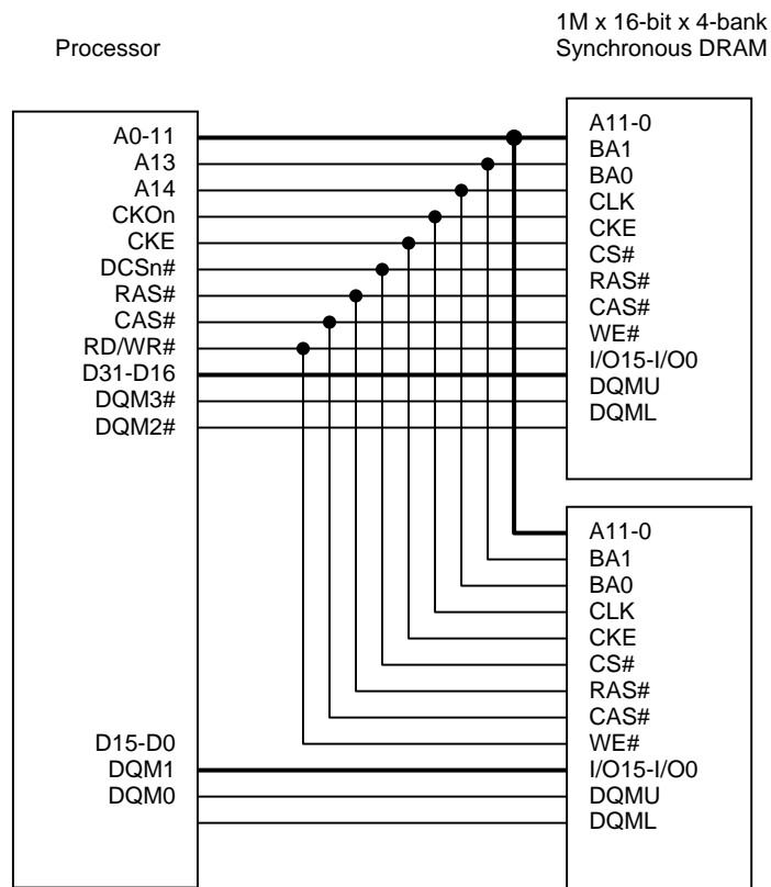
Figure 1-19 Example of Synchronous DRAM Chip Connection (2)
