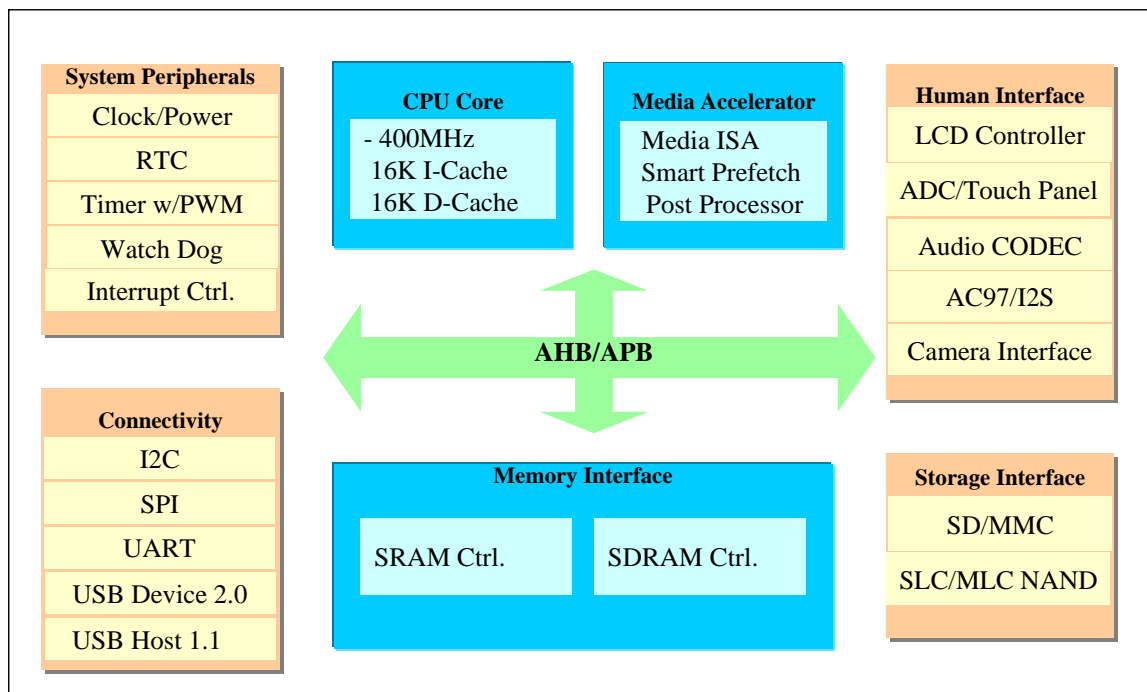
Figure 1-1 Jz4740 Diagram
