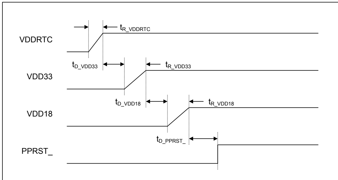
Figure 3-1 Power-On Timing Diagram
